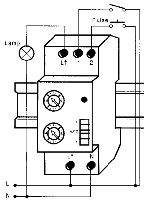
WIRING DIAGRAM
